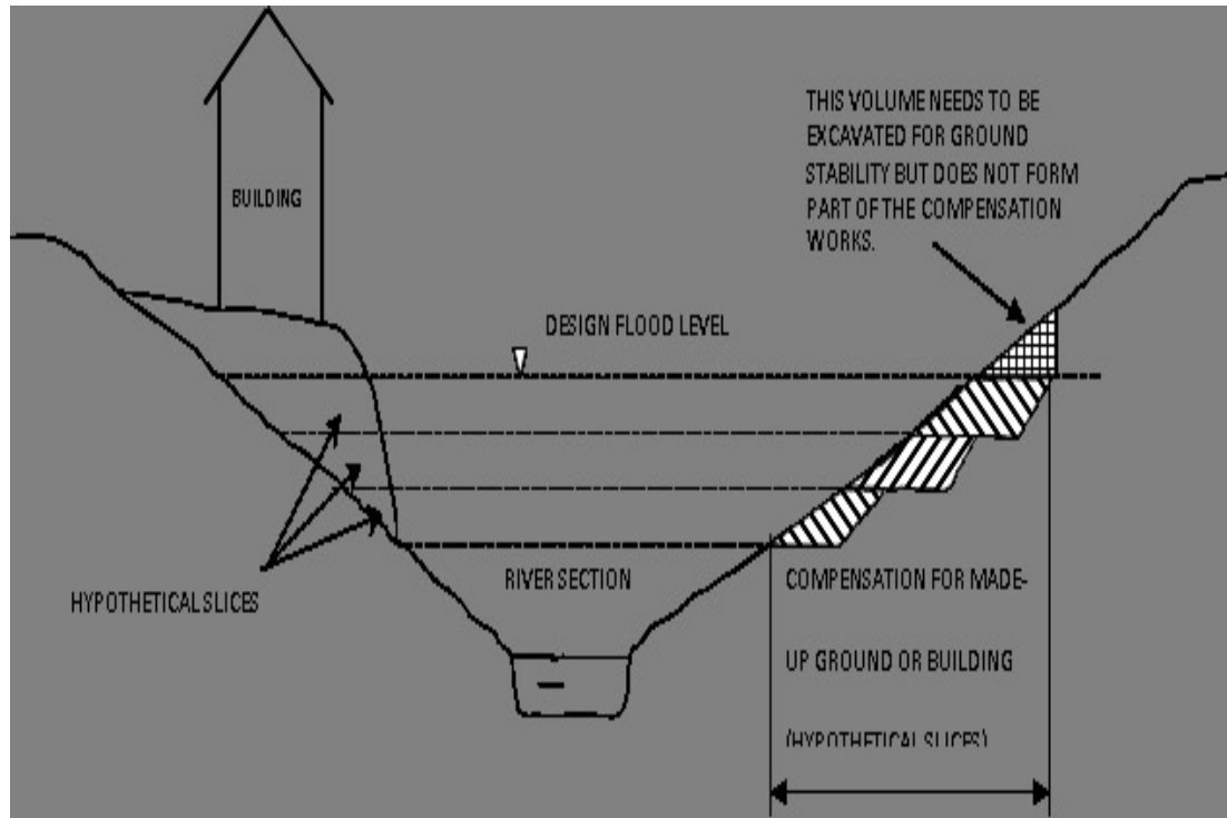
Figure 4 - Example of direct Floodplain Compensation Storage (Environment Agency 2009)
